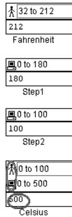
Fig. 5. An assertion conflict in Forms/3. The user wrote the assertion on the Celsius cell (0 to 100), which conflicts with the computer generated assertion (0 to 500). This prompts the user to check for errors in the cells' formulas [Burnett et al. 2003]. Original figure obtained from authors.
