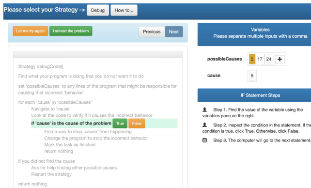
Figure 3: The strategy tracker, showing a conditional step of the debug strategy. The tracker acts as a scratchpad for relevant information and enforces the steps of the strategy.
