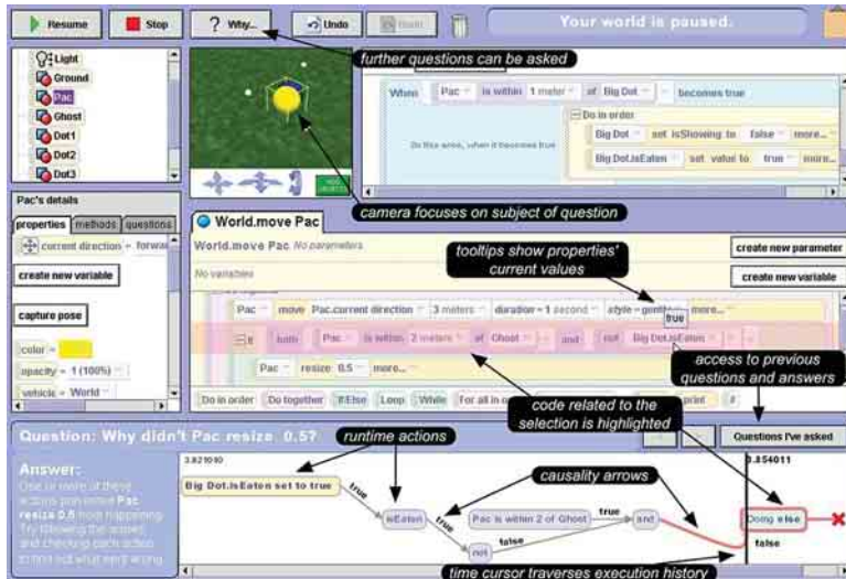
Figure 3. The Whyline's answer shows a visualization of the runtime actions that prevented Pac from resizing.
