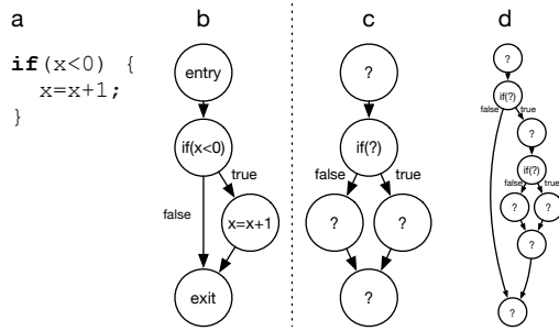
Figure 1: At label (a) a concrete program, then (b) its control flow graph (CFG), with specific conditions and assignments. At (c) a semantic CFG, (d) a composite semantic CFG, with ? placeholders.
